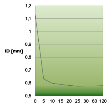
Performance of FEP QuickShrink™ 2.0
